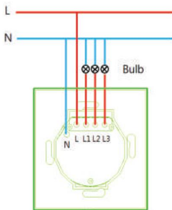
Lights wiring instruction (Eg:EU 3CH)
