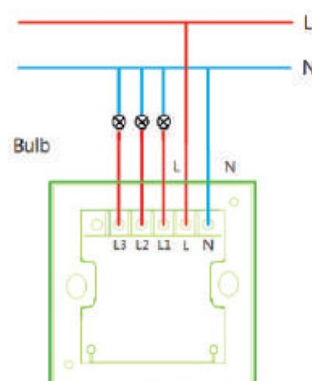
Lights wiring instruction (Eg:UK 3CH)
