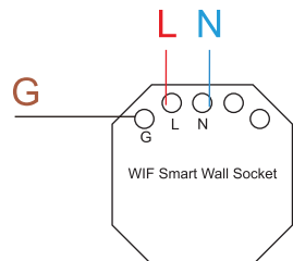
EU Wall Socket
