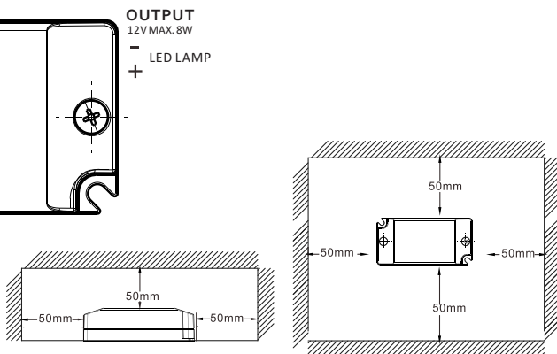
Mounting Location Dimension
