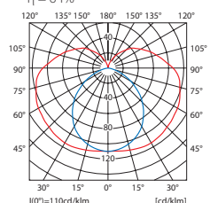
CO-C180 C90-C270 [cd/klm] GLORIA TL3011-30W
