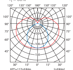
CO-C180 C90-C270 [cd/klm] GLORIA TL3011-36W
