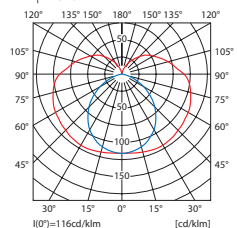
CO-C180 C90-C270 [cd/klm] GLORIA TL3011-18W
